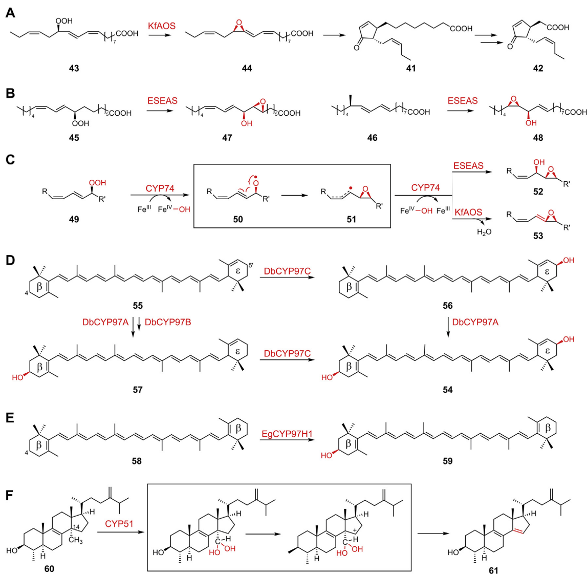
Figure 4 The reactions catalyzed by eukaryotic algal P450s and the related enzymatic mechanism (in box). (A) The oxylipin allene oxide ( 44 ) epoxidation catalyzed by KfAOS from the green microalgae Klebsormidium flaccidum during the formation of 41 and 42 . (B) The epoxidation reactions catalyzed by ESEAS from the brown algae Ectocarpus siliculosus . (C) The putative mechanisms of KfAOS and ESEAS. (D) The hydroxylation reactions of \alpha -carotene ( 55 ), \alpha -cryptoxanthin ( 56 ) and zeinoxanthin ( 57 ) catalyzed by DbCYP97C from the green algae Dunaliella bardawil during the biosynthesis of lutein ( 54 ). (E) The hydroxylation reaction of \beta -cryptoxanthin ( 59 ) catalyzed by EgCYP97H1 from Euglena gracilis . (F) The CYP51 mediated 14 \alpha -demethylation reaction during sterol biosynthesis.
