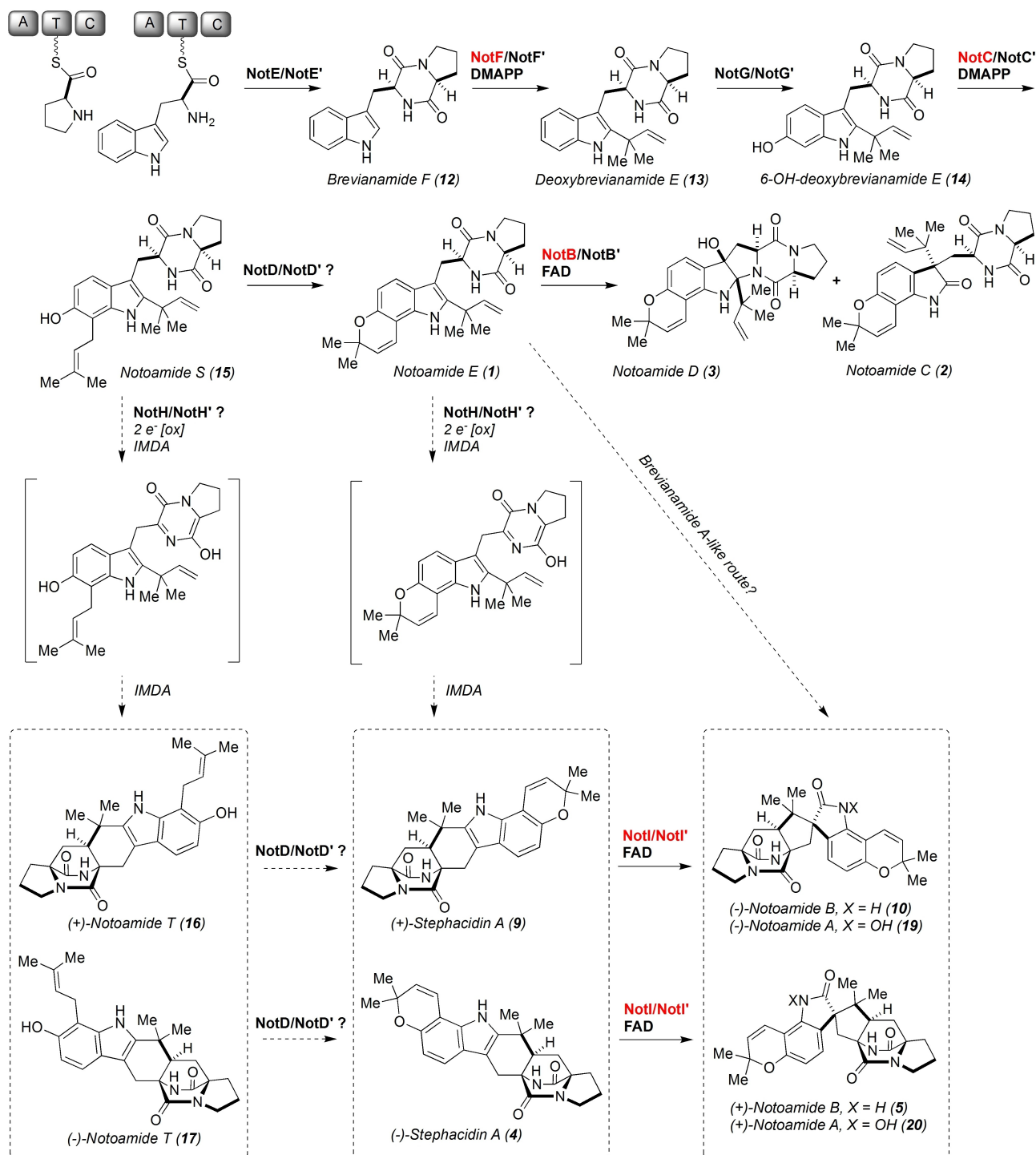
Scheme 2. Proposed (-)/(+) notoamide A (19 and 20) biosynthetic pathways. The functions of enzymes highlighted in red have been experimentally confirmed. The terminal N-hydroxylation to generate 19 and 20 is catalyzed by an additional enzyme subsequent to spirocyclization.
