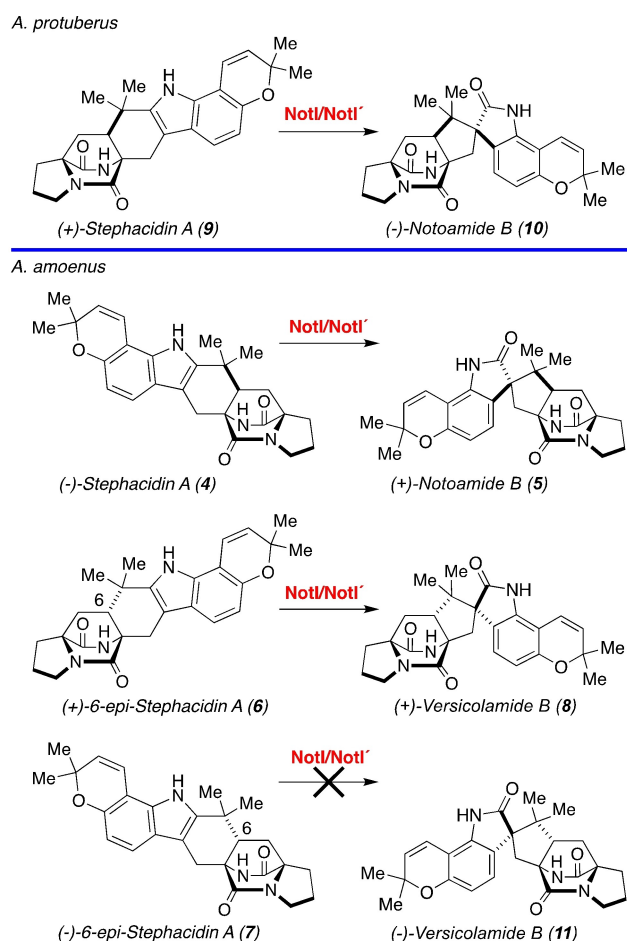
Scheme 1. Reactions catalyzed by NotI/NotI' in vitro and in the respective native fungal species.
